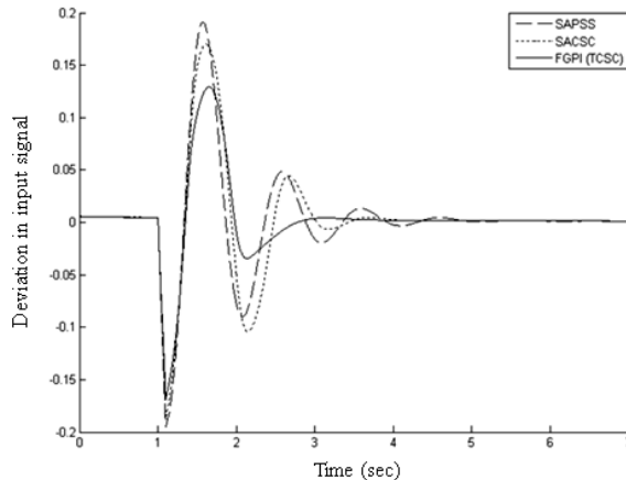
Fig. 12: Input signal response for case 3
