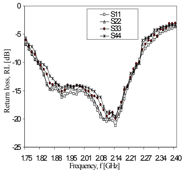
Fig. 6: Return loss for 4x1 LIEH shaped BMPAA
