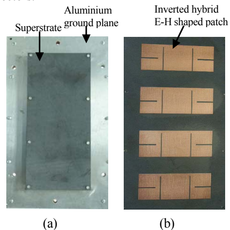
Fig. 5: The fabricated 4×1 LIEH shaped BMPAA: (a) top view, (b) inside view showing inverted element
