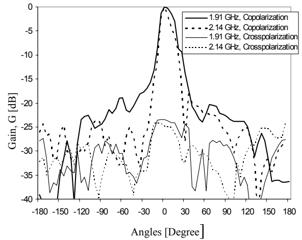
Fig. 7: Measured E-plane radiation patterns for the LIEH shaped BMPAA at 1.91 GHz and 2.14 GHz
