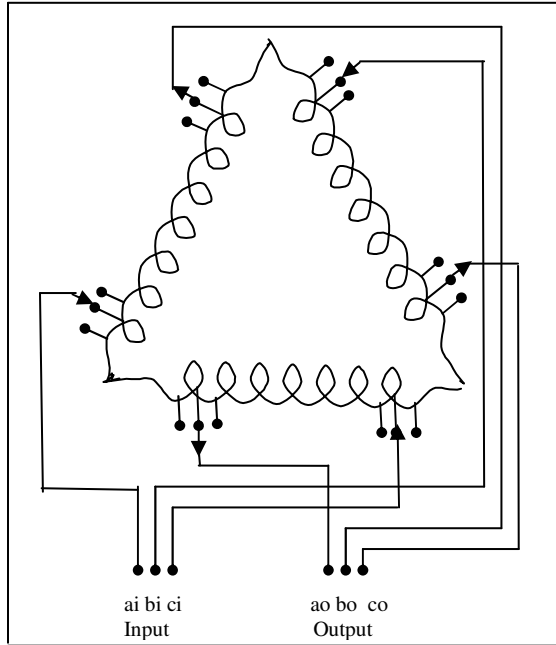
Fig. 3: Delta connected tapped autotransformer
