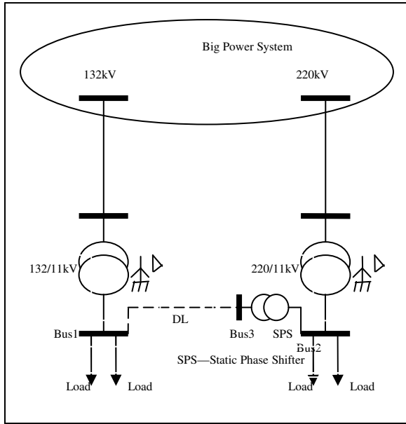
Fig.1: Distribution system
