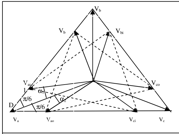
Fig. 4: No-load phasor diagram
