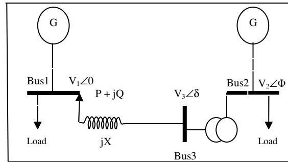
Fig. 2: Equivalent circuit
